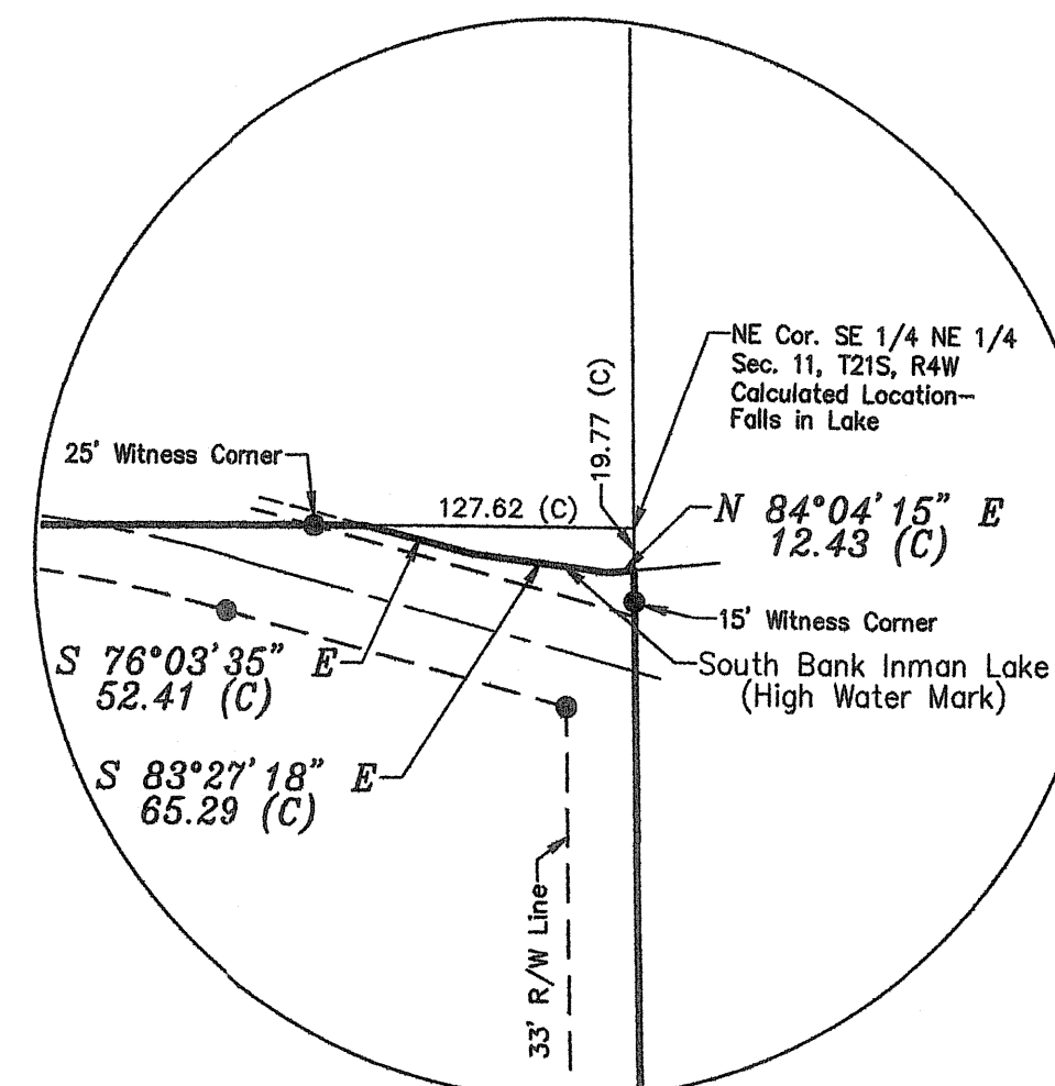
DETAIL Scale 1"=100'
