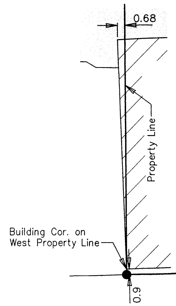
Detail 1 Not to Scale
