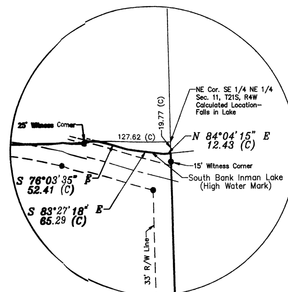
DETAIL Scale 1"=100'
